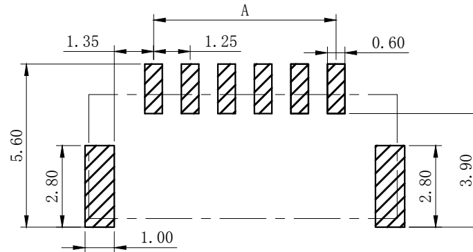
PCB LAYOUT
